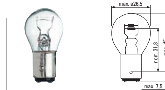
P21/5W - BAY15d
