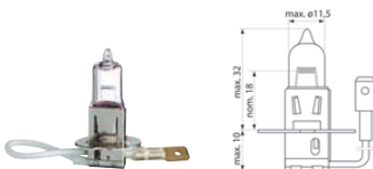
H3 - PK22s
