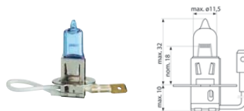
H3 - PK22s
