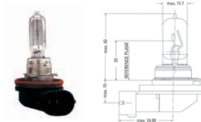
H9 - PGJ19-5
