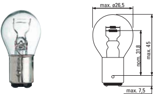
P21/4W - BAZ15d
