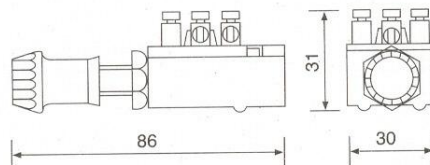
Headlight Push - Pull Switch With Metal Shaft Code Nr : E2062B
