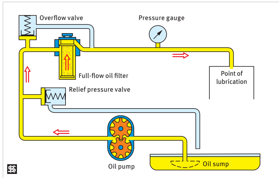
Forced-feed lubrication
