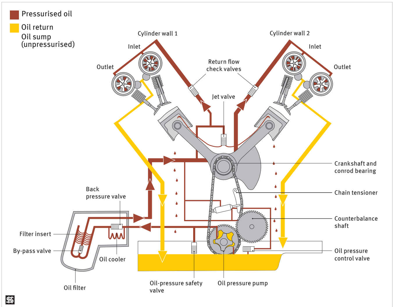
Oil circulation
