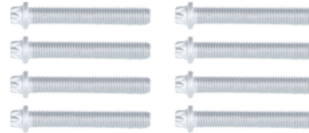
M10x1,5x60 mm
