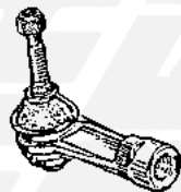
6 - 713407 (Fil. gambo S / Stem thread LH 12x1,75) 7 - 713408 (Fil. gambo D / Stem thread RH 12x1,75)
