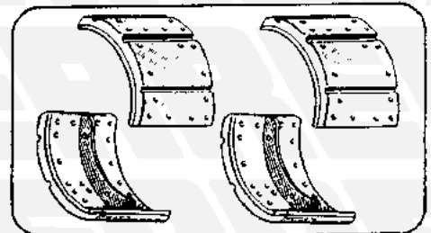
711350 c/ceppi normali / with std linings 14
