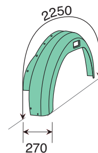
641/200 d/rh/rechts 641/201 s/lh/links cabina bassa-lunga low cab, long type langes Fhs.
