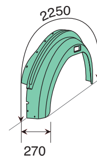
641/198 d/rh/rechts 641/199 s/lh/links cabina alta- lunga high cab, long type langes Fhs. - 80 mm erhöht
