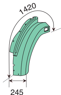
641/214 d/rh/rechts 641/215 s/lh/links cabina alta-corta. high cab, short type kurzes Fhs. - 80 mm erhöht
