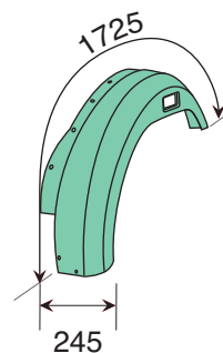
641/204 d/rh/rechts 641/205 s/lh/links cabina bassa-media low cab, medium type mittell. Fhs.
