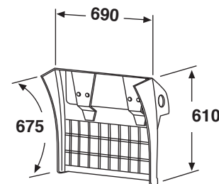
B TGX/543 d/s-rh/lh rechts/links
