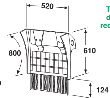
B TGX/513 d/s-rh/lh rechts/links
